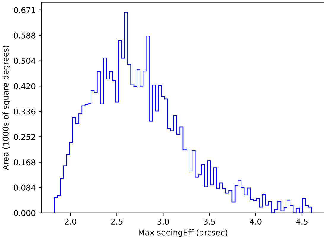
ddf_acor_sf25_lsf40_lsr20_v3.4_10yrs WFD r band: Max seeingEff
