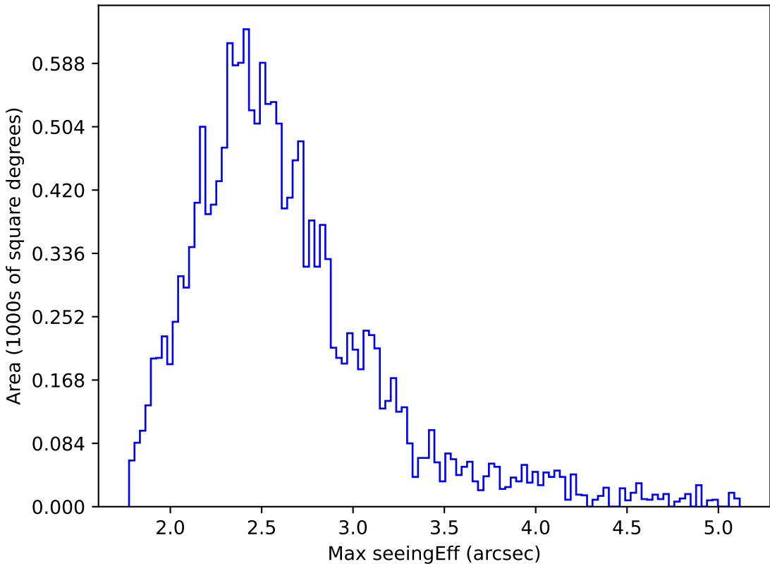
ddf_acor_sf25_lsf40_lsr20_v3.4_10yrs WFD i band: Max seeingEff
