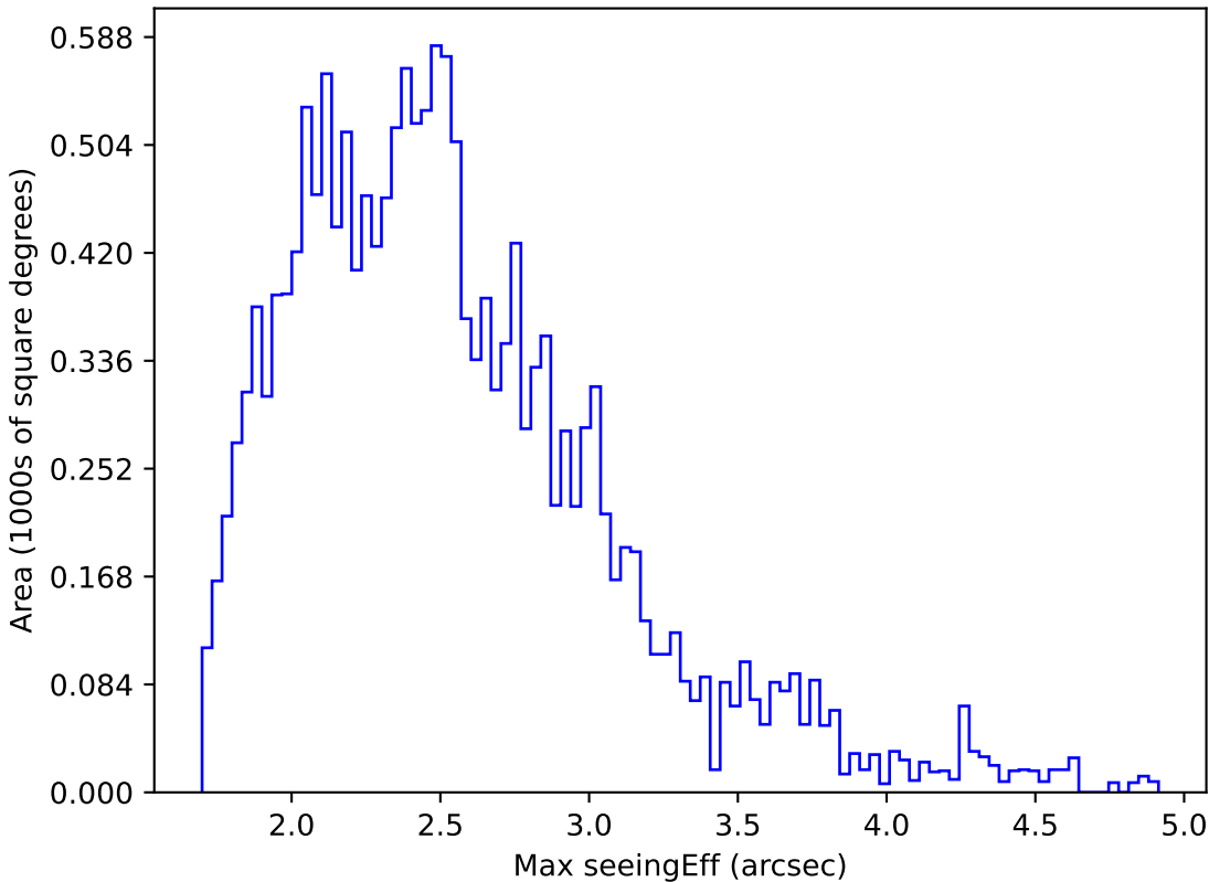
ddf_acor_sf25_lsf40_lsr20_v3.4_10yrs WFD g band: Max seeingEff
