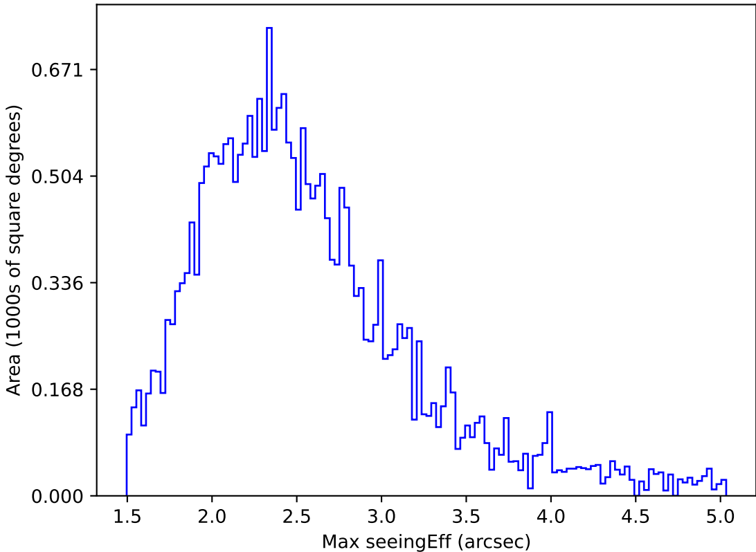
ddf_acor_sf25_lsf40_lsr20_v3.4_10yrs All sky z band: Max seeingEff
