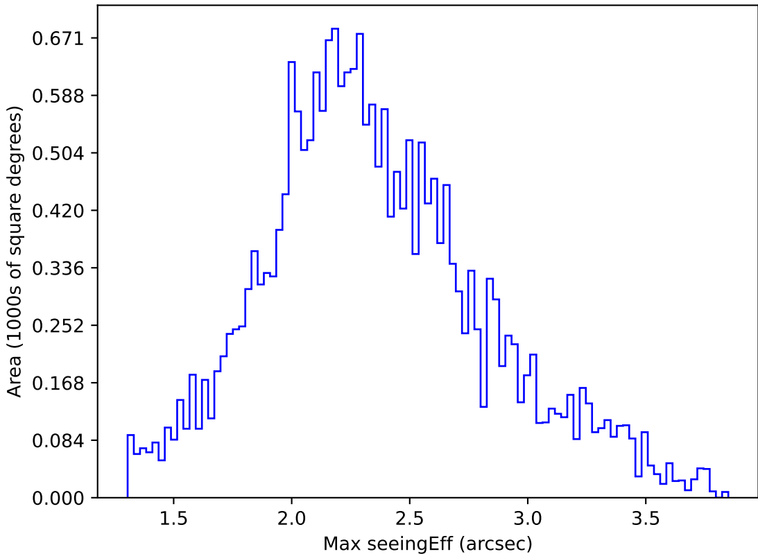
ddf_acor_sf25_lsf40_lsr20_v3.4_10yrs All sky u band: Max seeingEff
