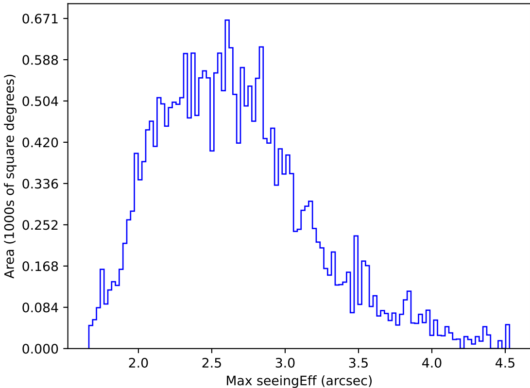
ddf_acor_sf25_lsf40_lsr20_v3.4_10yrs All sky r band: Max seeingEff
