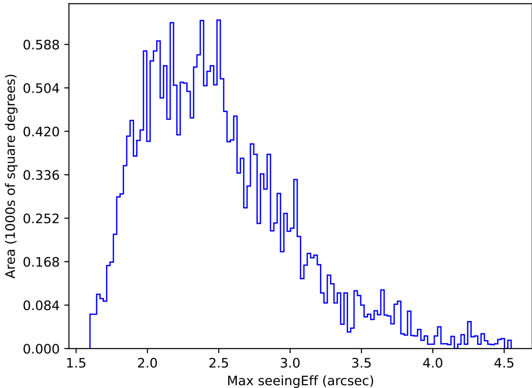
ddf_acor_sf25_ls40_lsr20_v3.4_10yrs All sky g band: Max seeingEff
