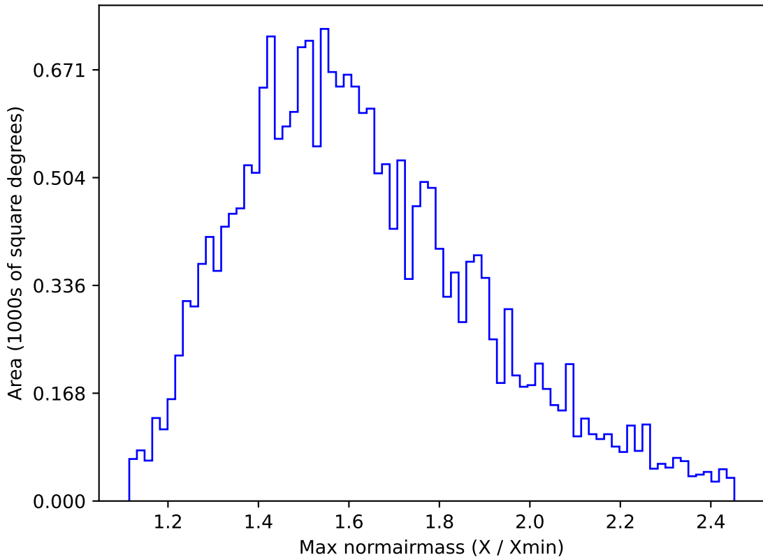
ddf_acor_sf25_lsf40_lsr20_v3.4_10yrs All sky u band: Max normairmass
