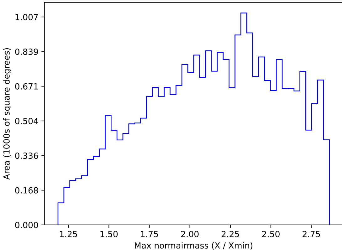
ddf_acor_sf25_ls40_lsr20_v3.4_10yrs All sky i band: Max normairmass
