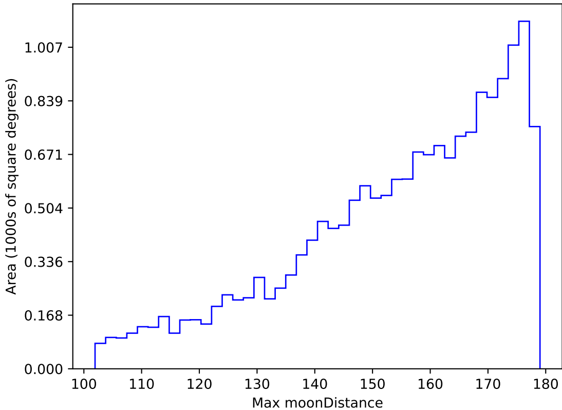
ddf_acor_sf25_lsf40_lsr20_v3.4_10yrs WFD u band: Max moonDistance
