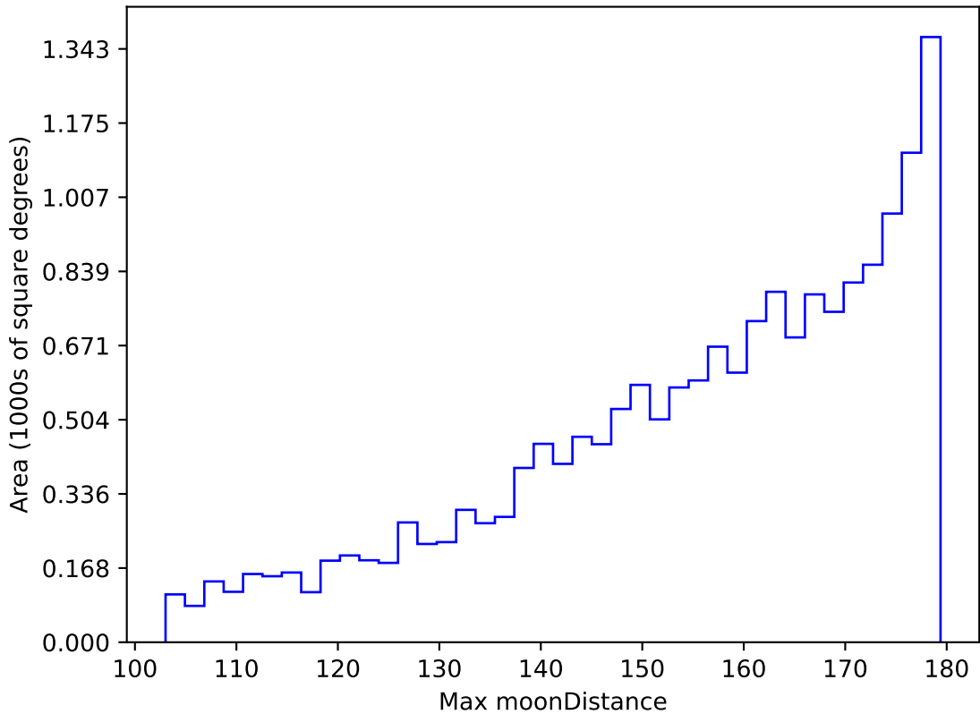
ddf_acor_sf25_lsf40_lsr20_v3.4_10yrs WFD i band: Max moonDistance
