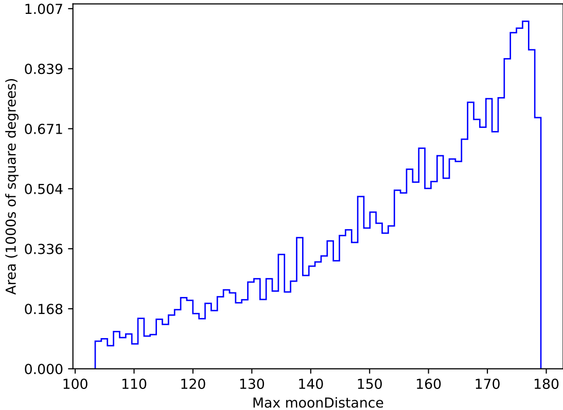
ddf_acor_sf25_lsf40_lsr20_v3.4_10yrs All sky g band: Max moonDistance
