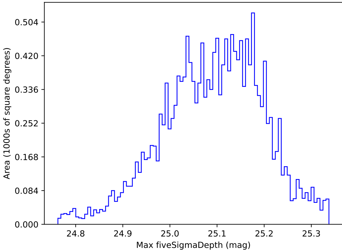
ddf_acor_sf25_lsf40_lsr20_v3.4_10yrs WFD all bands: Max fiveSigmaDepth
