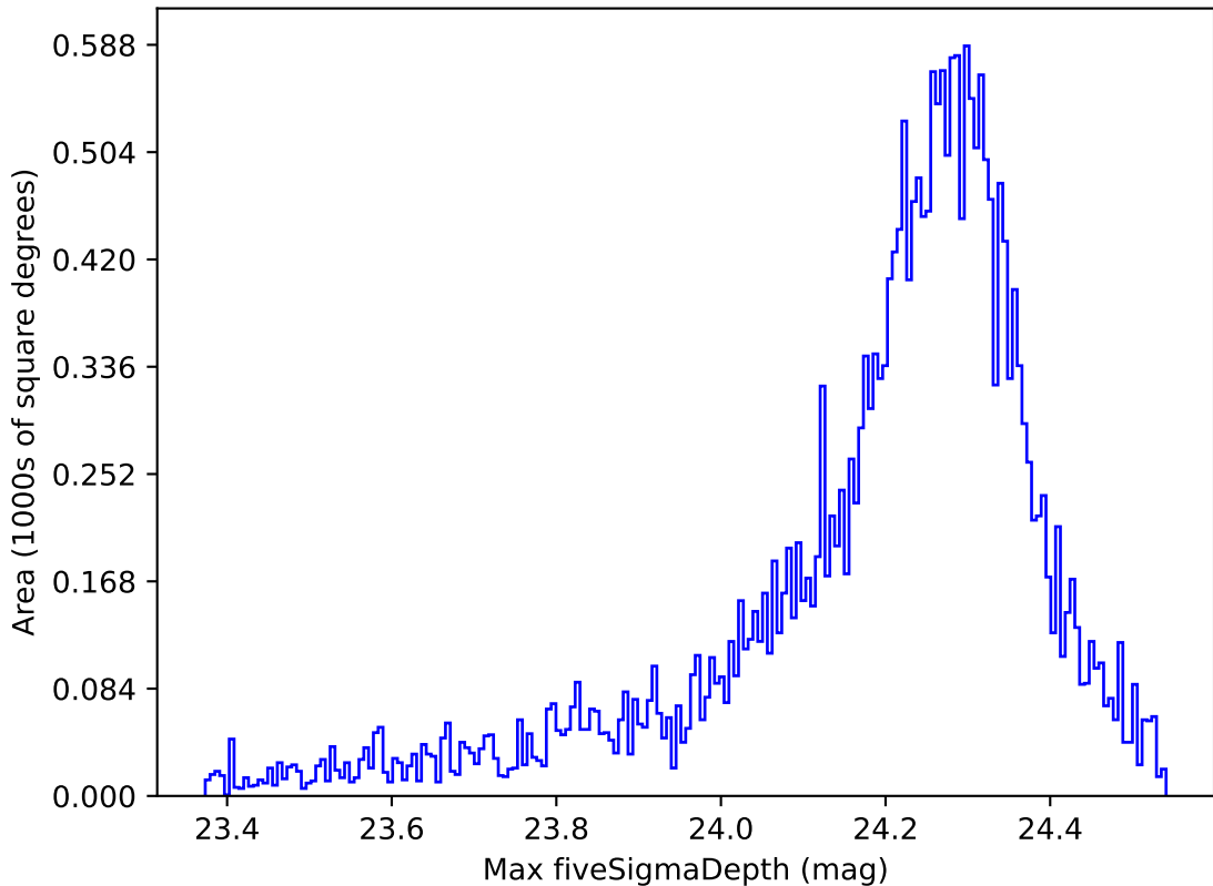
ddf_acor_sf25_lsf40_lsr20_v3.4_10yrs All sky i band: Max fiveSigmaDepth
