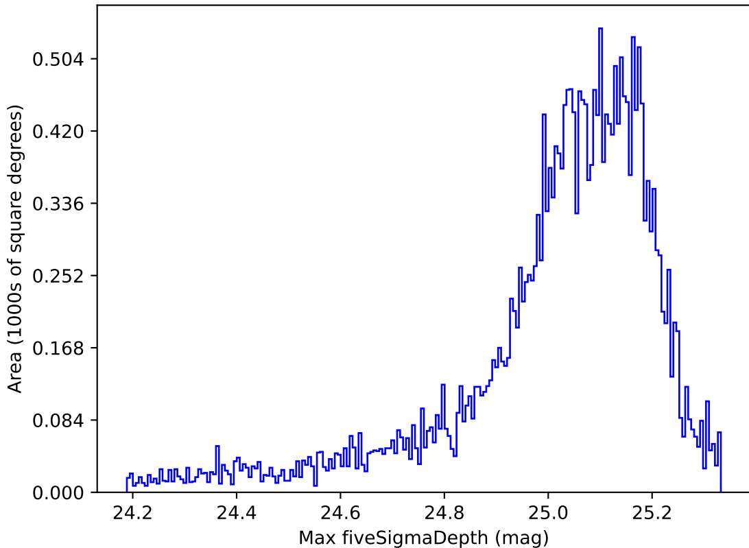
ddf_acor_sf25_lsf40_lsr20_v3.4_10yrs All sky g band: Max fiveSigmaDepth
