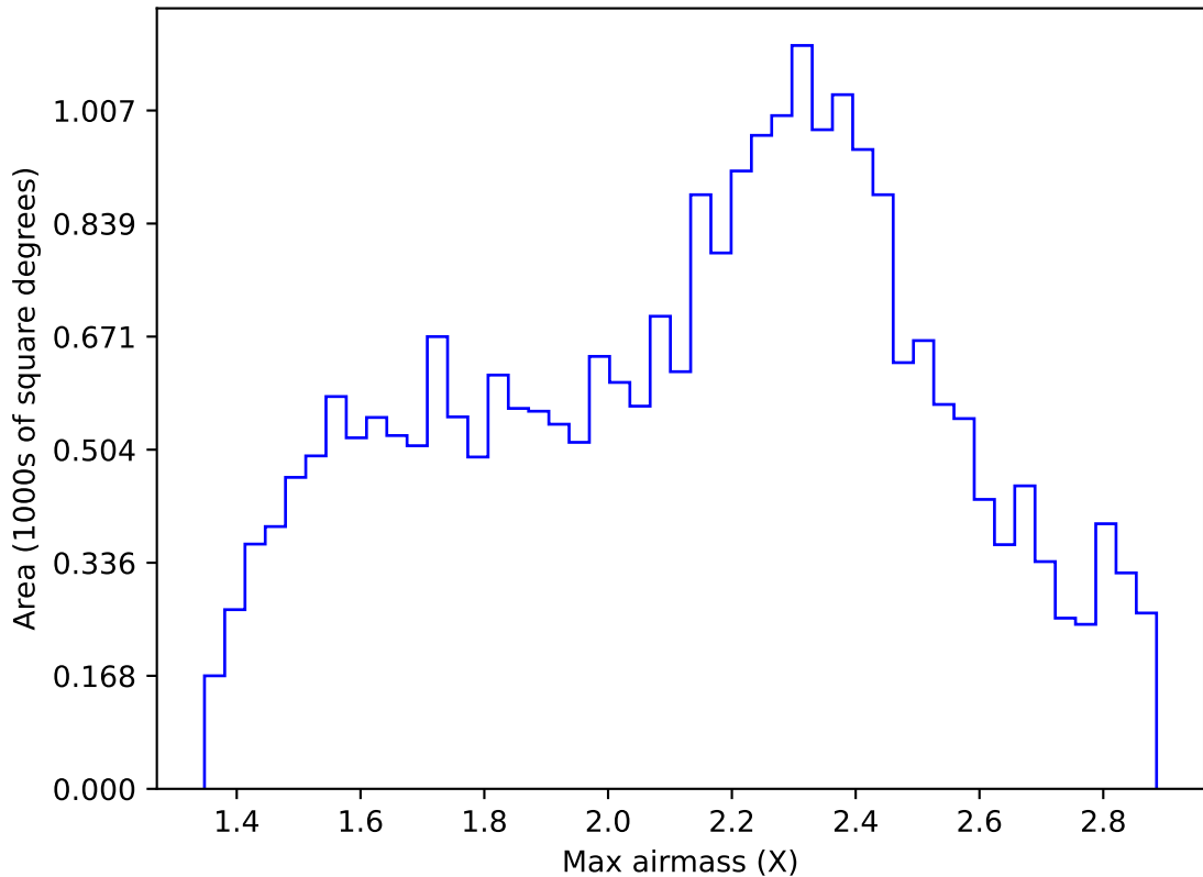
ddf_acor_sf25_lsf40_lsr20_v3.4_10yrs Yr 1 all bands: Max airmass
