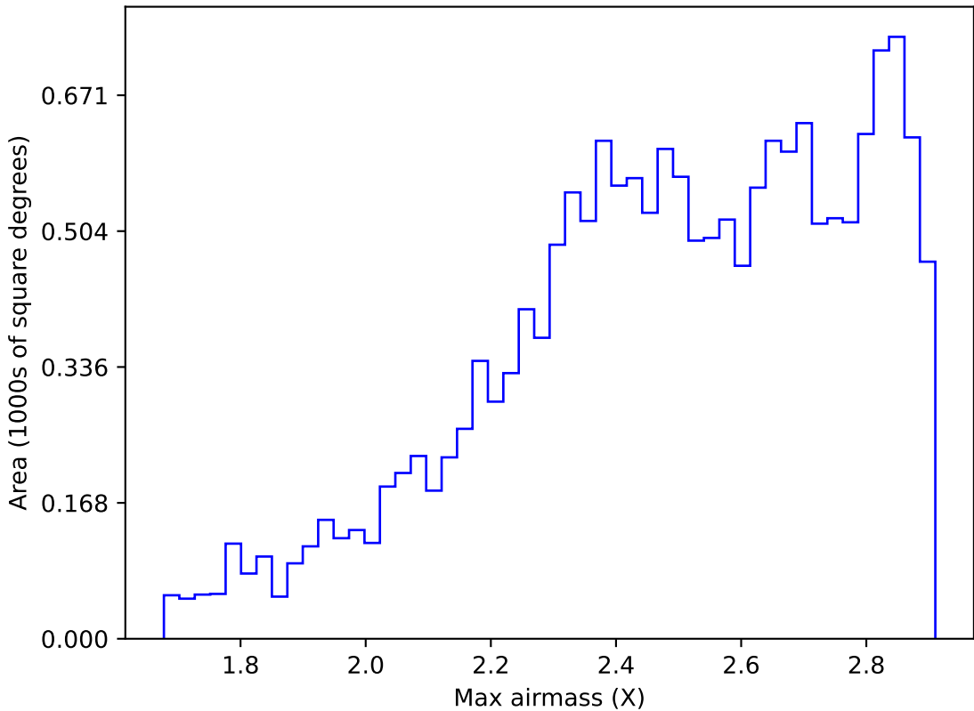
ddf_acor_sf25_lsf40_lsr20_v3.4_10yrs WFD i band: Max airmass
