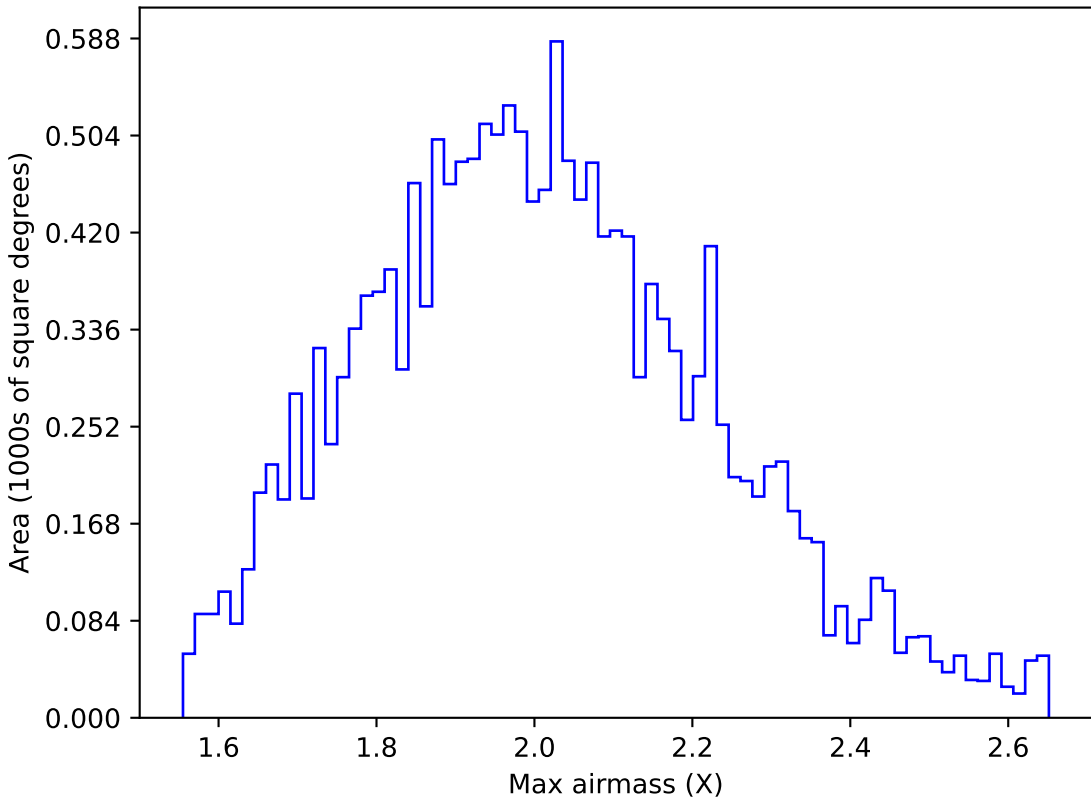
ddf_acor_sf25_lsf40_lsr20_v3.4_10yrs WFD g band: Max airmass
