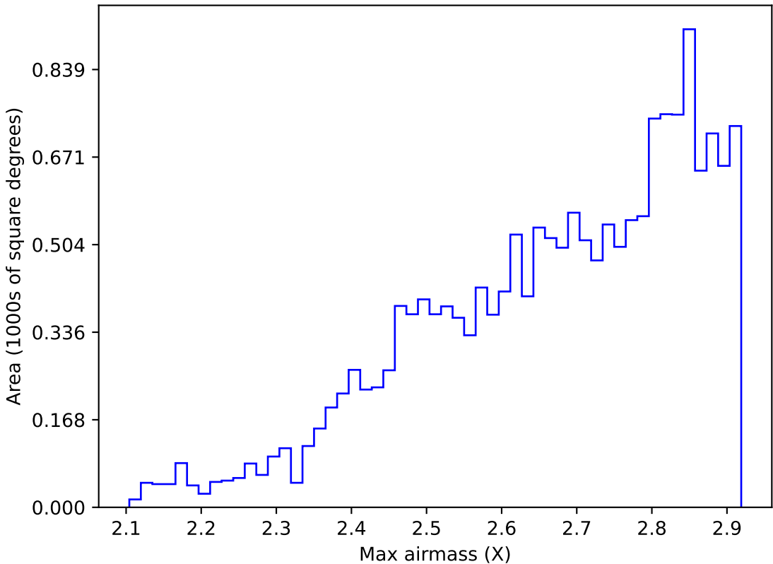
ddf_acor_sf25_lsf40_lsr20_v3.4_10yrs WFD all bands: Max airmass
