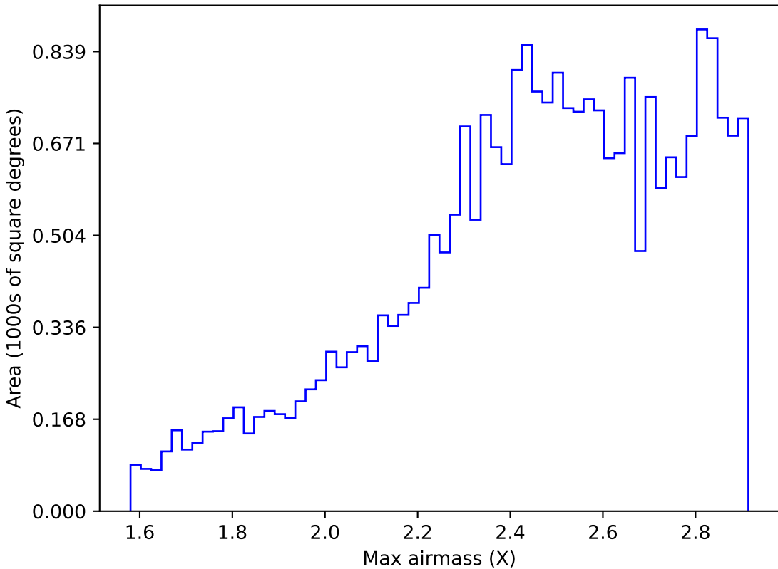
ddf_acor_sf25_lsf40_lsr20_v3.4_10yrs All sky z band: Max airmass
