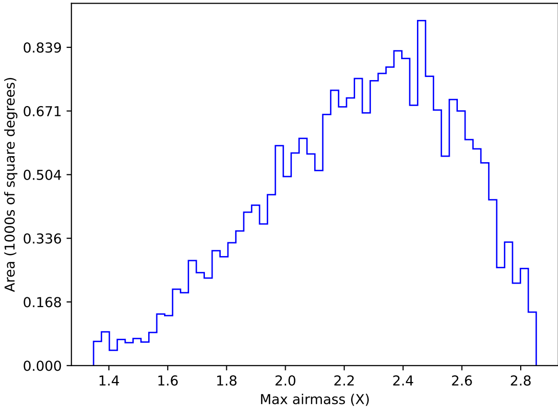
ddf_acor_sf25_lsf40_lsr20_v3.4_10yrs All sky y band: Max airmass
