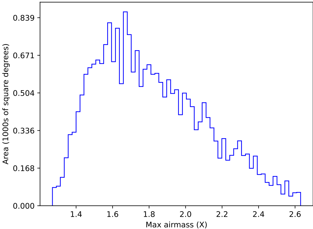
ddf_acor_sf25_lsf40_lsr20_v3.4_10yrs All sky u band: Max airmass
