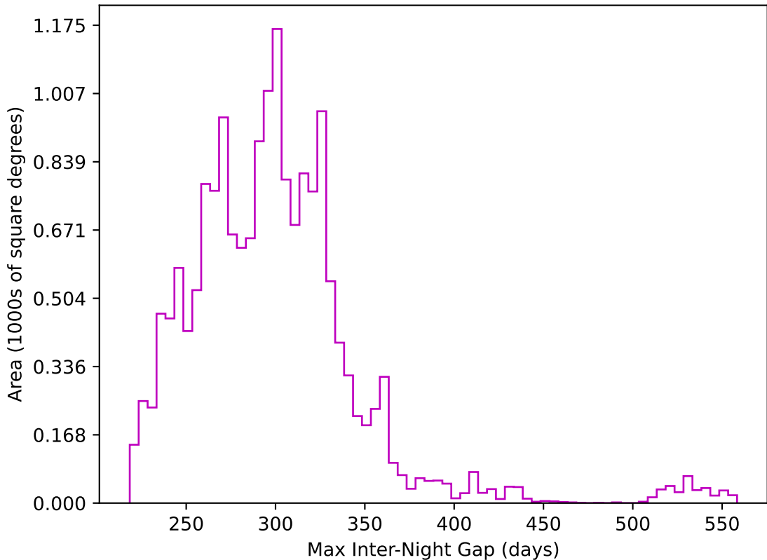
ddf_acor_sf25_lsf40_lsr20_v3.4_10yrs WFD z band: Max Inter-Night Gap
