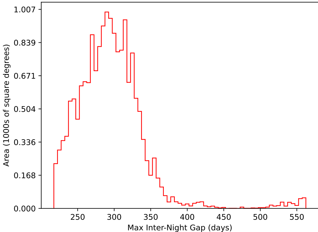
ddf_acor_sf25_ls40_lsr20_v3.4_10yrs WFD i band: Max Inter-Night Gap
