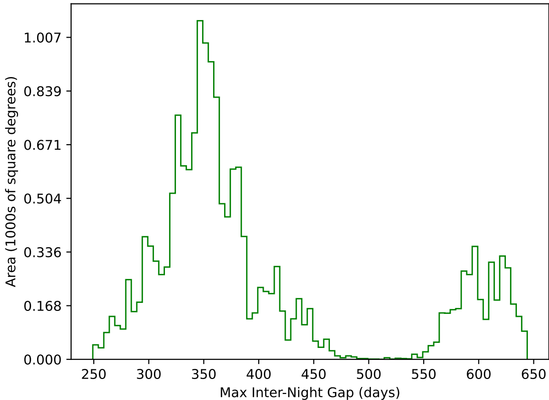
ddf_acor_sf25_lsf40_lsr20_v3.4_10yrs WFD g band: Max Inter-Night Gap
