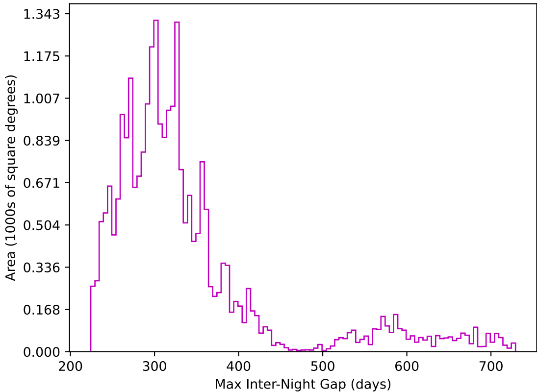
ddf_acor_sf25_lsf40_lsr20_v3.4_10yrs All sky z band: Max Inter-Night Gap
