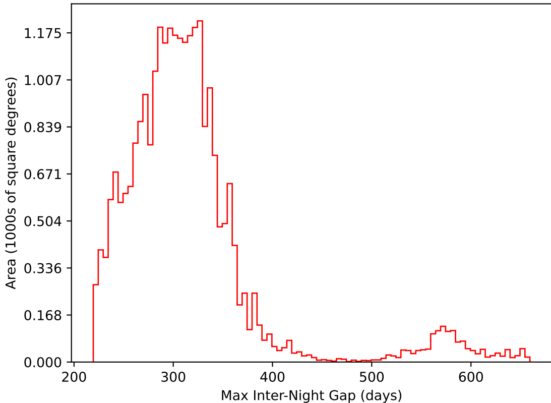
ddf_acor_sf25_lsf40_lsr20_v3.4_10yrs All sky i band: Max Inter-Night Gap
