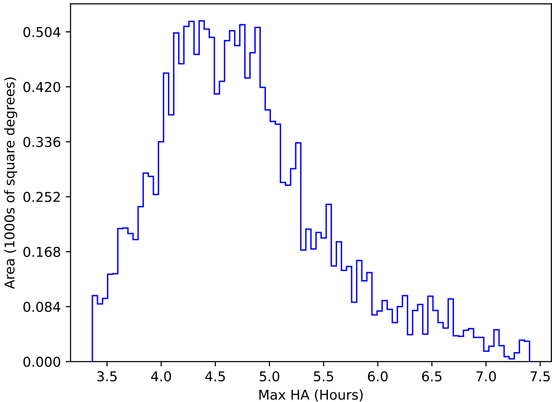
ddf_acor_sf25_lsf40_lsr20_v3.4_10yrs WFD y band: Max HA
