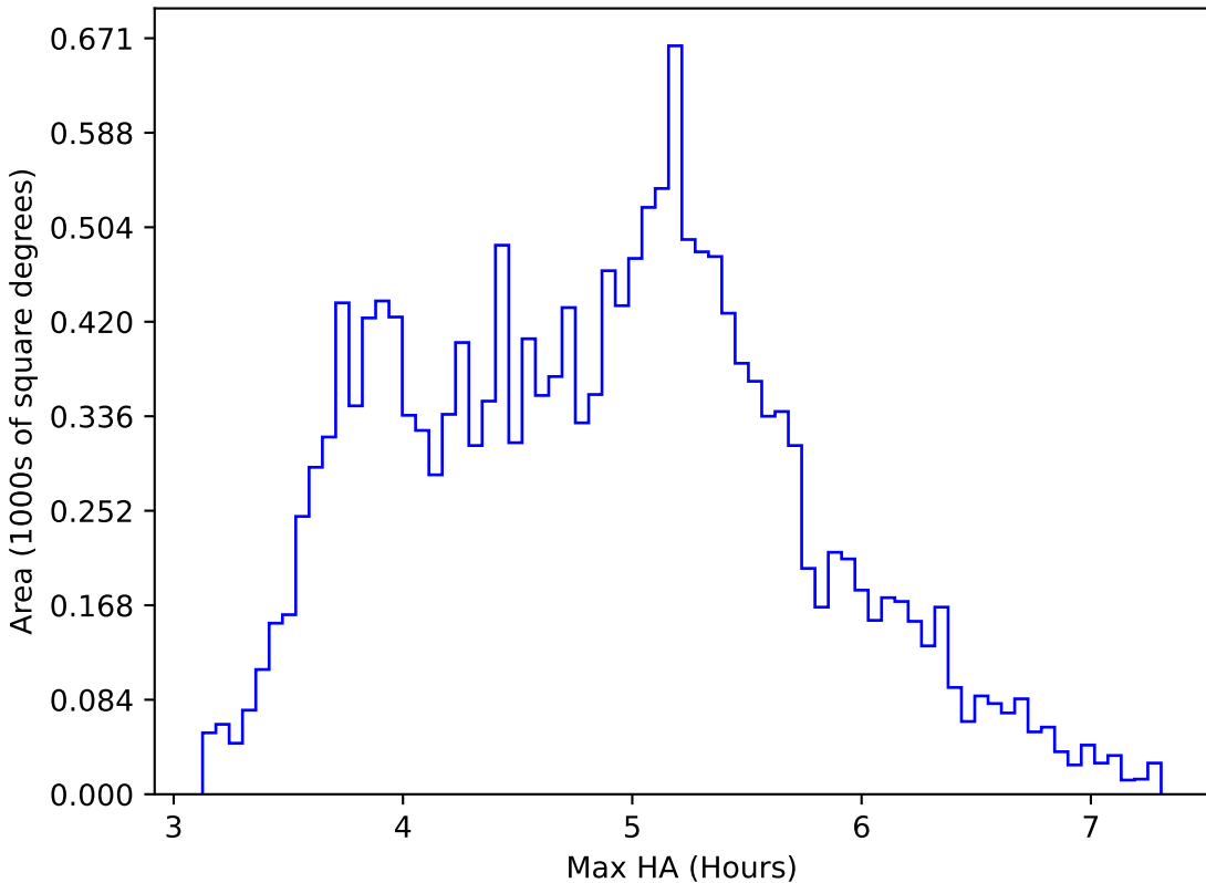
ddf_acor_sf25_lsf40_lsr20_v3.4_10yrs WFD i band: Max HA
