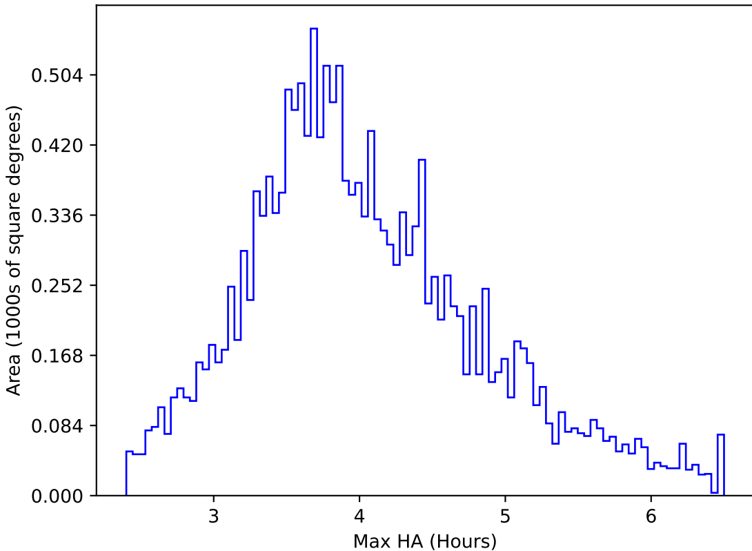
ddf_acor_sf25_lsf40_lsr20_v3.4_10yrs WFD g band: Max HA
