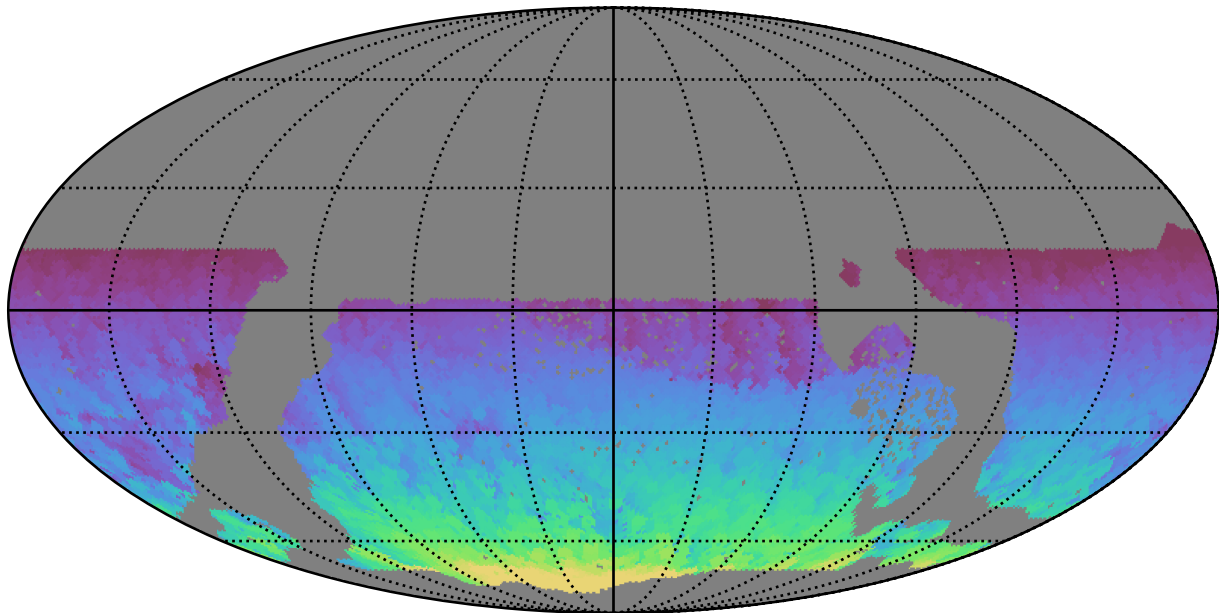
ddf_acor_sf25_lsf40_lsr20_v3.4_10yrs WFD all bands: Max HA
