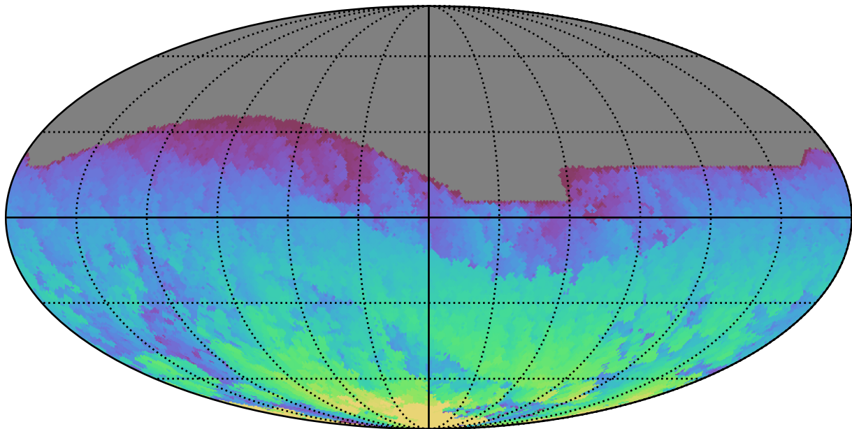
ddf_acor_sf25_lsf40_lsr20_v3.4_10yrs All sky z band: Max HA
