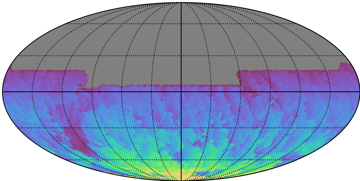
ddf_acor_sf25_lsf40_lsr20_v3.4_10yrs All sky y band: Max HA
