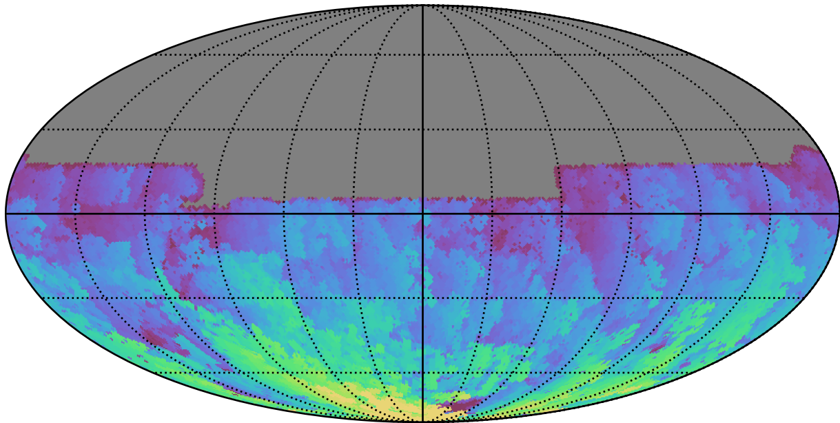
ddf_acor_sf25_lsf40_lsr20_v3.4_10yrs All sky u band: Max HA
