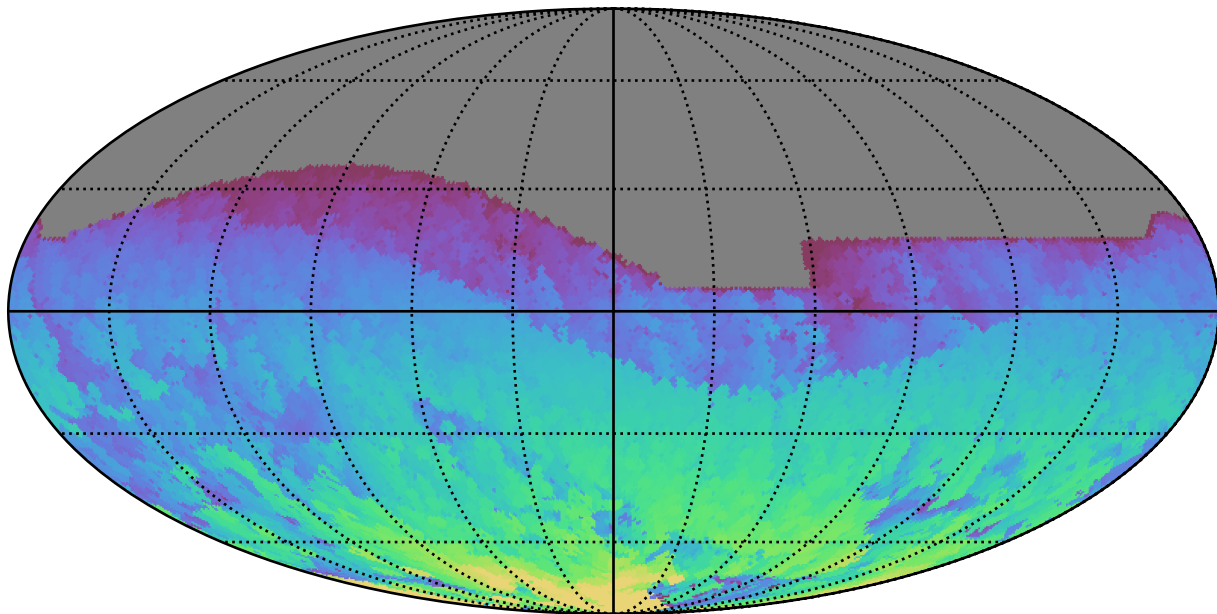
ddf_acor_sf25_lsf40_lsr20_v3.4_10yrs All sky i band: Max HA
