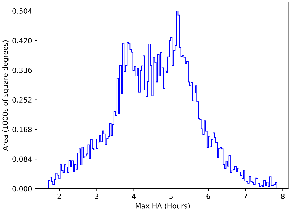
ddf_acor_sf25_lsf40_lsr20_v3.4_10yrs All sky i band: Max HA
