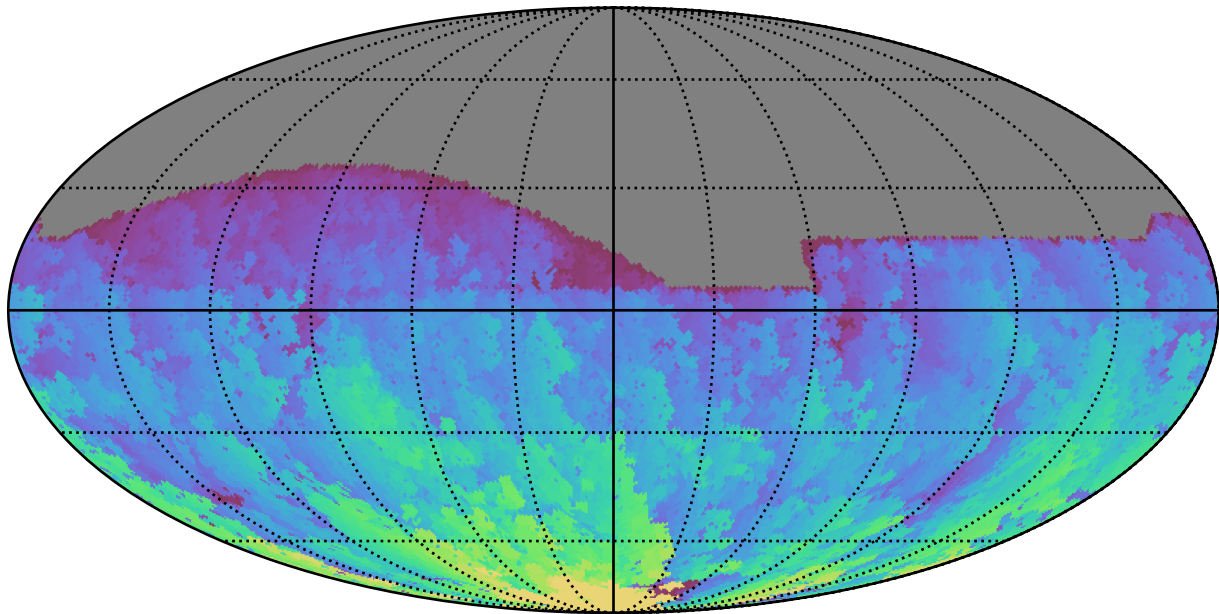
ddf_acor_sf25_lsf40_lsr20_v3.4_10yrs All sky g band: Max HA
