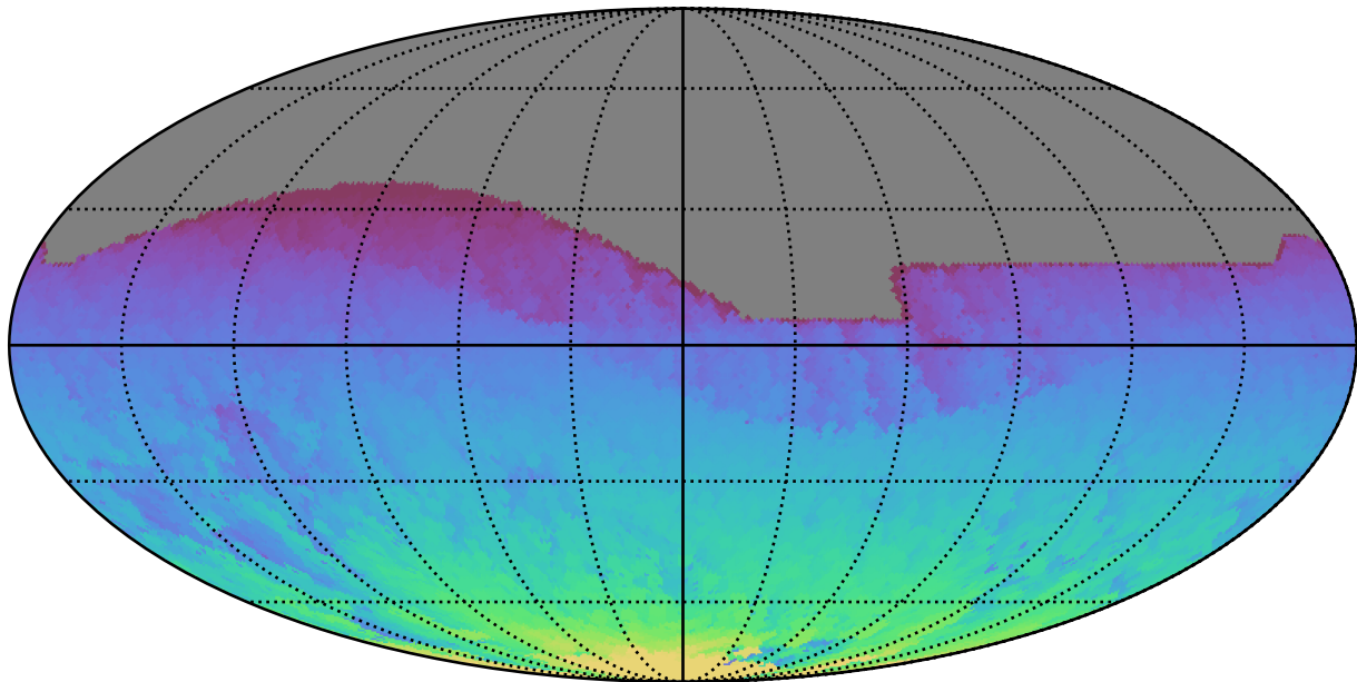
ddf_acor_sf25_lsf40_lsr20_v3.4_10yrs All sky all bands: Max HA
