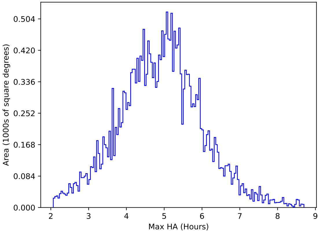
ddf_acor_sf25_lsf40_lsr20_v3.4_10yrs All sky all bands: Max HA
