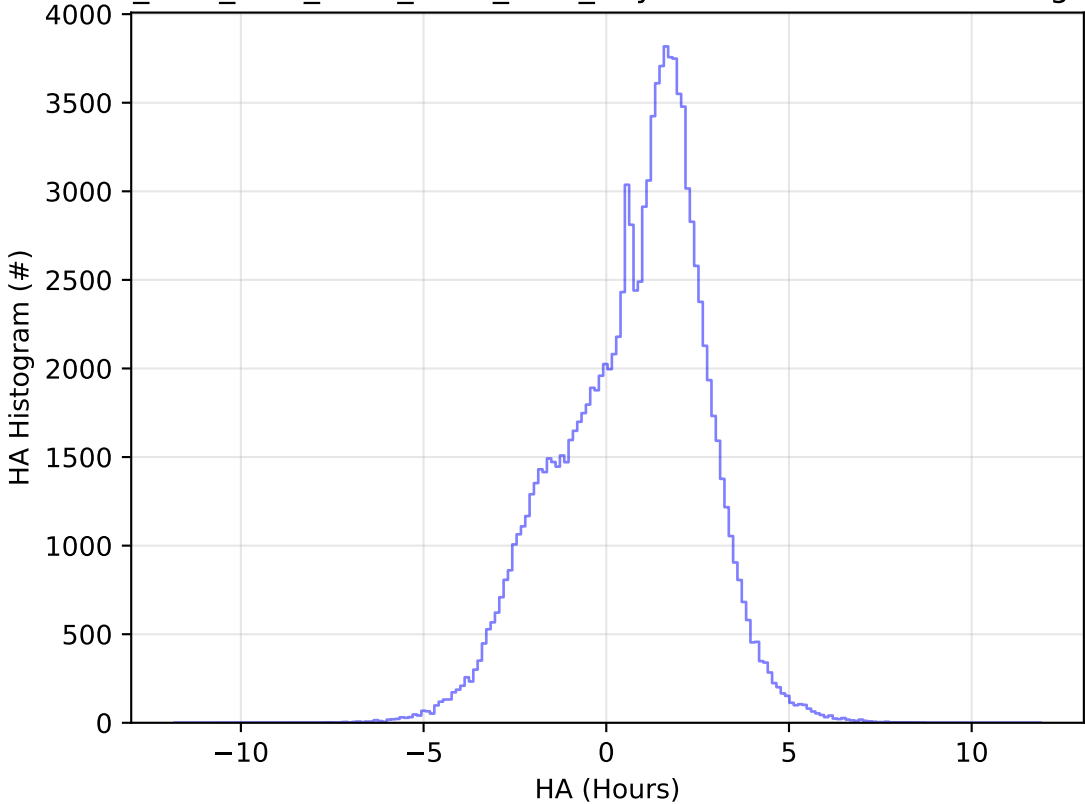
ddf_acor_sf25_lsf40_lsr20_v3.4_10yrs WFD u band: HA Histogram
