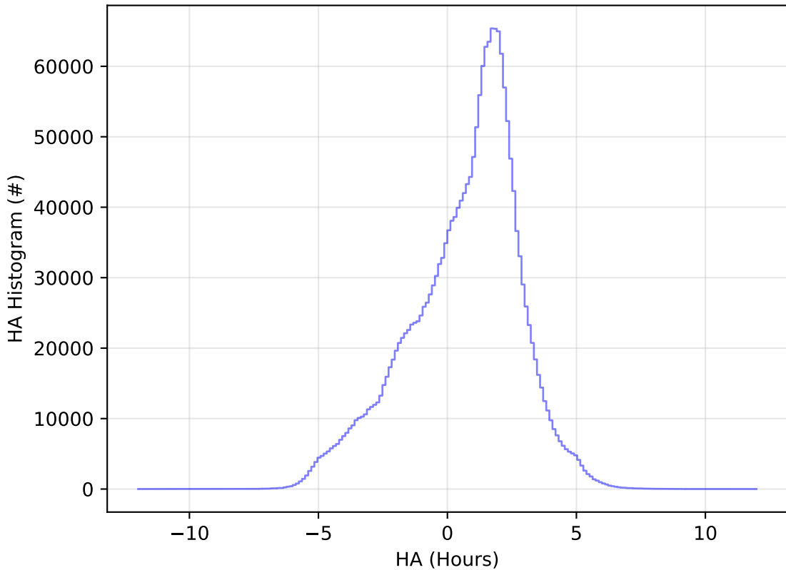
ddf_acor_sf25_lsf40_lsr20_v3.4_10yrs WFD all bands: HA Histogram
