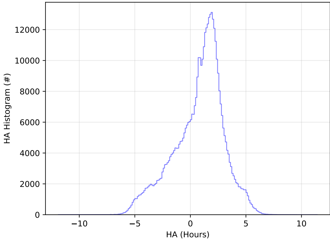
ddf_acor_sf25_lsf40_lsr20_v3.4_10yrs All sky z band: HA Histogram
