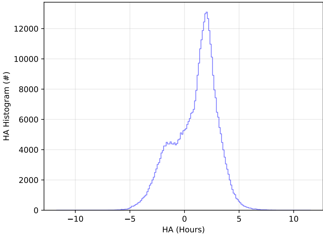
ddf_acor_sf25_lsf40_lsr20_v3.4_10yrs All sky y band: HA Histogram
