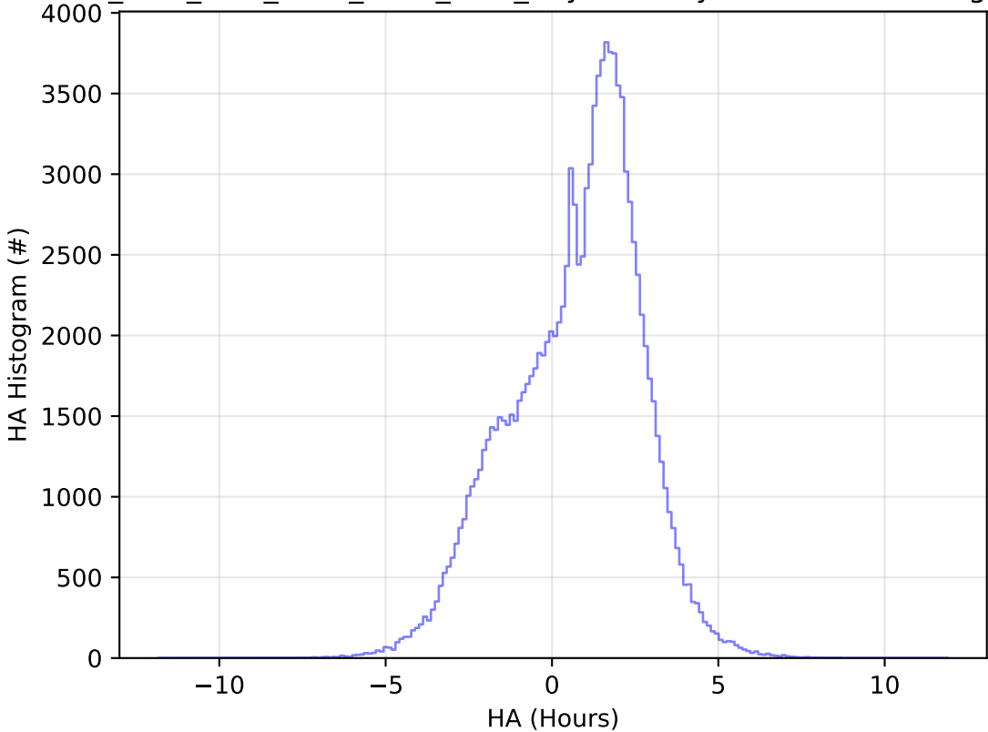
ddf_acor_sf25_lsf40_lsr20_v3.4_10yrs All sky u band: HA Histogram
