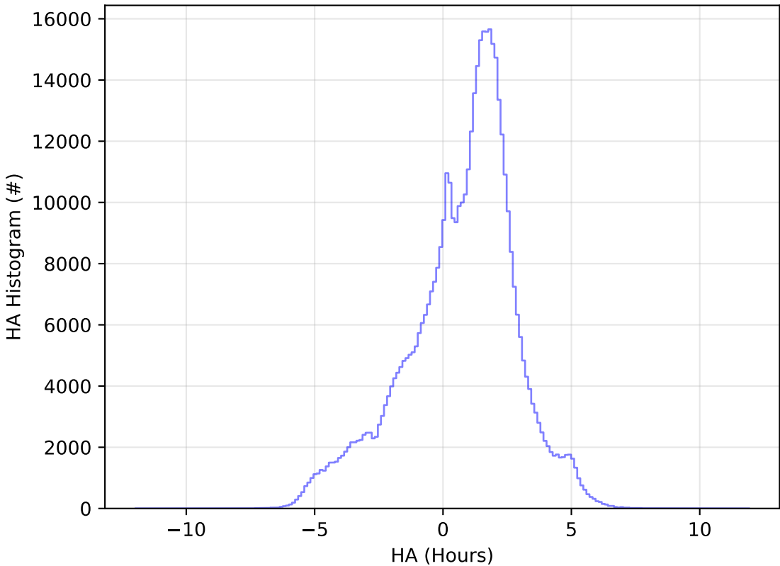
ddf_acor_sf25_lsf40_lsr20_v3.4_10yrs All sky i band: HA Histogram
