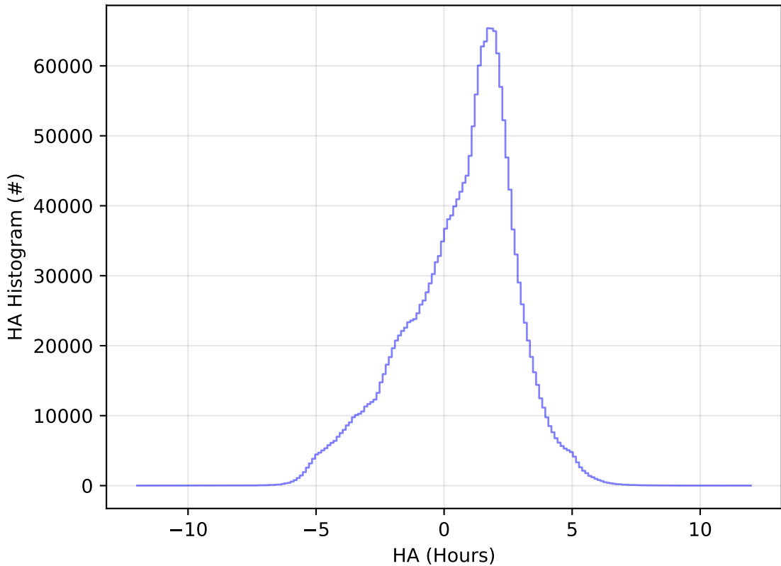
ddf_acor_sf25_lsf40_lsr20_v3.4_10yrs All sky all bands: HA Histogram
