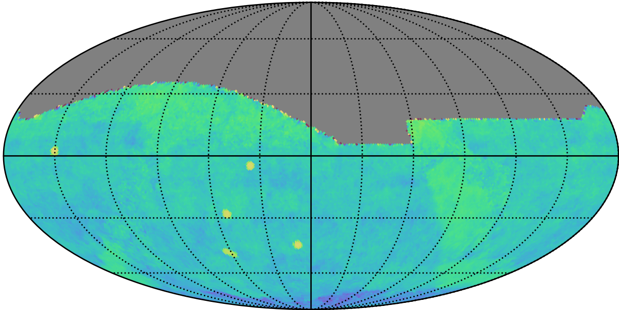
ddf_acor_sf25_lsf40_lsr20_v3.4_10yrs gri All sky: Fraction of visits in pairs (10-60 min)
