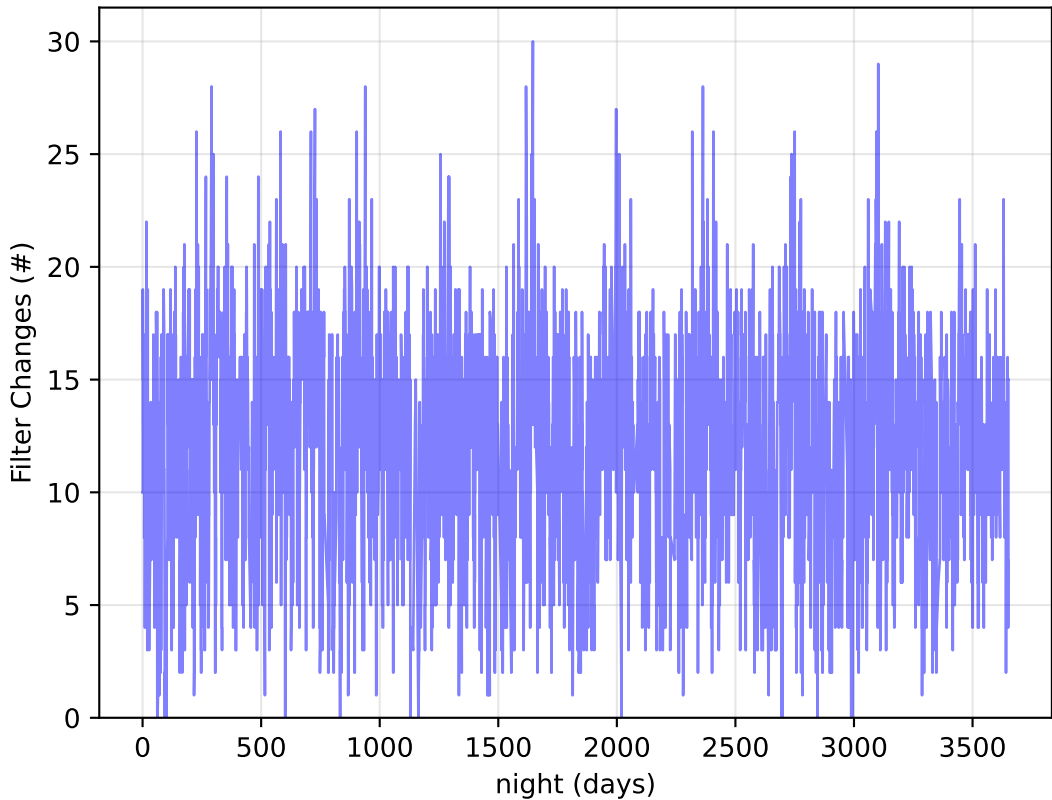
ddf_acor_sf25_Isf40_Isr20_v3.4_10yrs Per Night: Filter Changes
