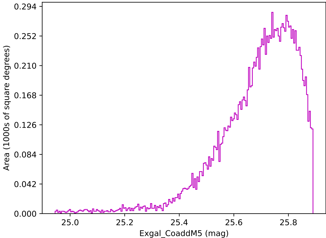
ddf_acor_sf25_lsf40_lsr20_v3.4_10yrs WFD z band: Exgal_CoaddM5
