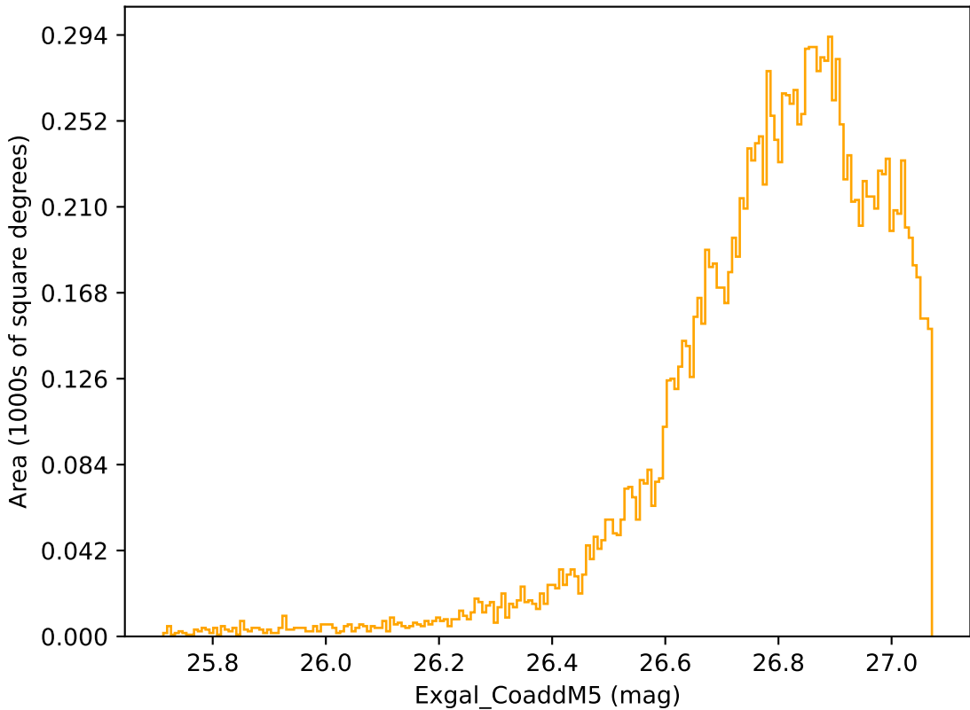
ddf_acor_sf25_lsf40_lsr20_v3.4_10yrs WFD r band: Exgal_CoaddM5
